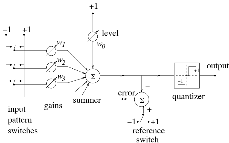
Figure 3.5: The Adaline.
