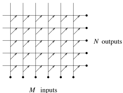
Figure 11.1: Connections between M input and N output neurons.
