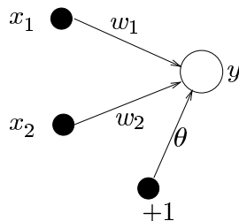
Figure 3.1: Single layer network with one output and two inputs.
