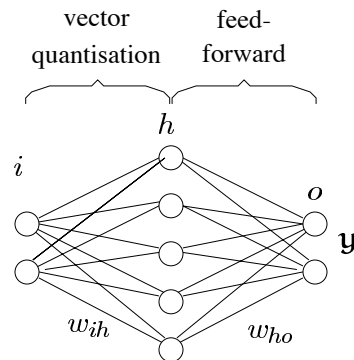
Figure 6.6: A network combining a vector quantisation layer with a 1-layer feed-forward neural network. This network can be used to approximate functions from \mathbb{R}^2 to \mathbb{R}^2 , the input space \mathbb{R}^2 is discretised in 5 disjoint subspaces.
